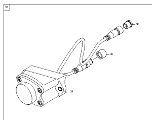
ETB-0000011038, Czujnik Argus (SRG)
