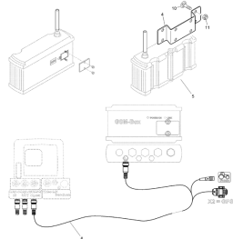
ETB-001164, Modem GSM CCI
