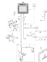
ETB-001147, ISOBUS CCI
